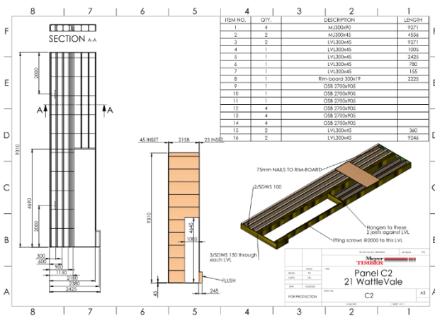
Cassette Production Drawing
