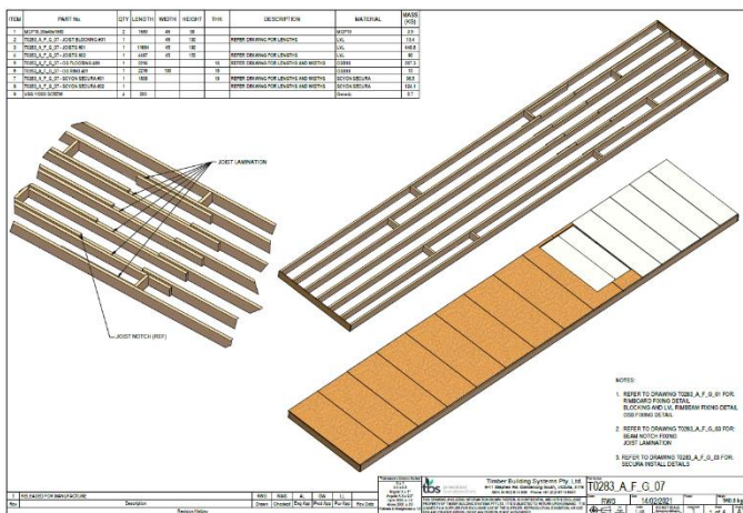
Cassette Production Drawing
