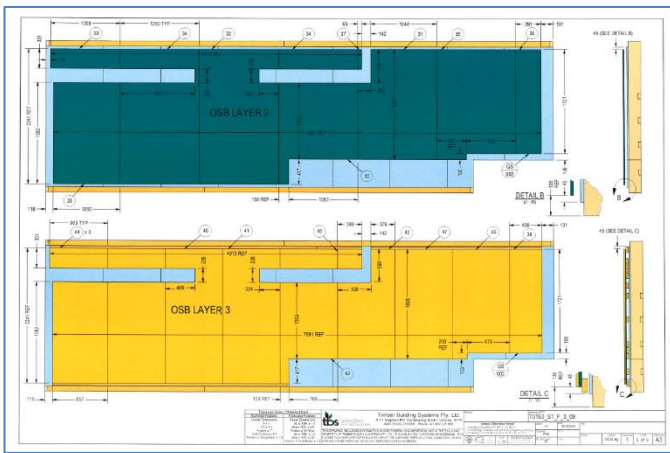
Production Drawing
