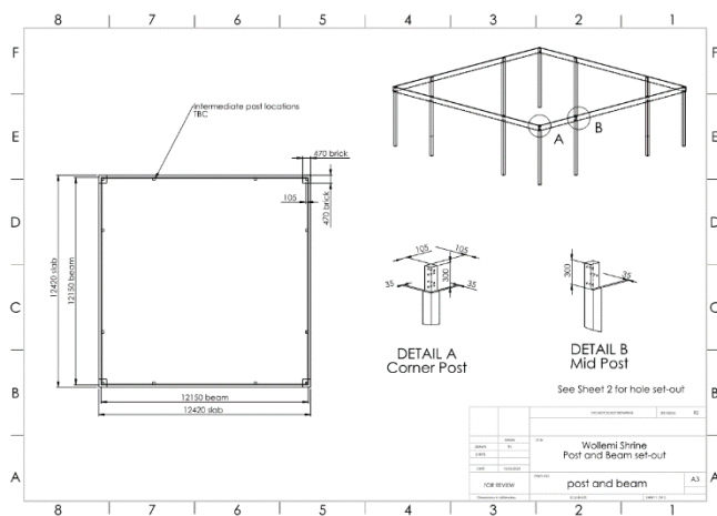
Post and Beam Production Drawings
