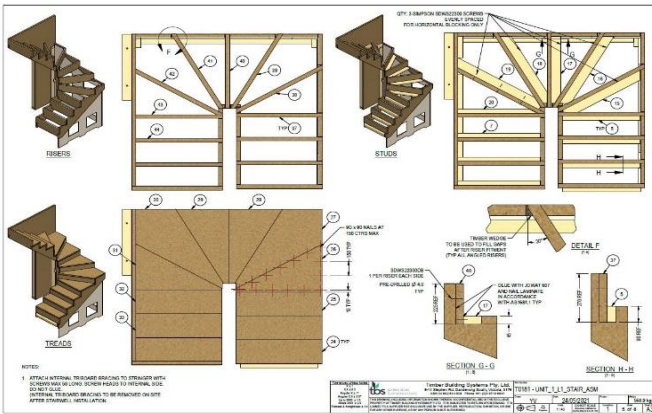
Detailed Drawings – illustrating the complex staircase
