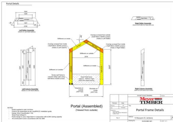
Portal Frame drawing
