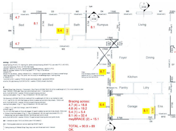
Double meyBRACE solution
