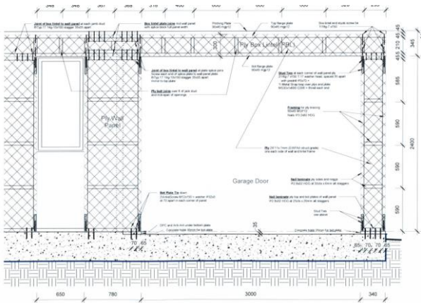
1 PBL Ply Box Lintel brace wall (hh) 1:20 Proposed Engineering
