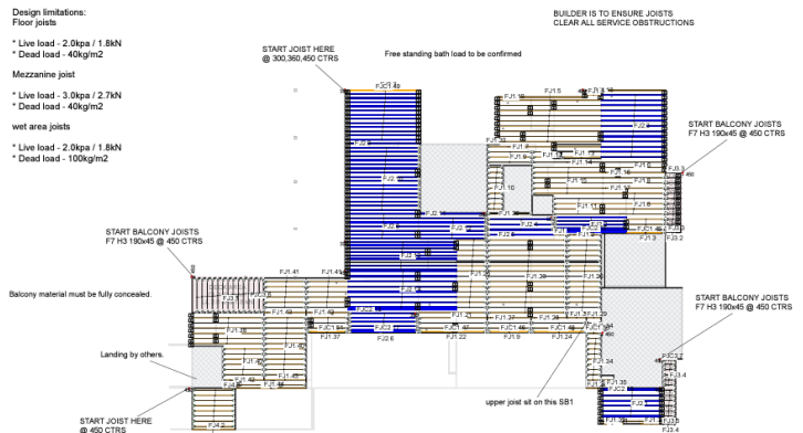
Floor joist layout
