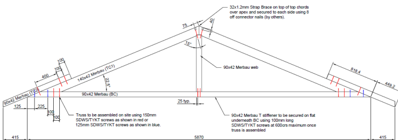
Truss detail
