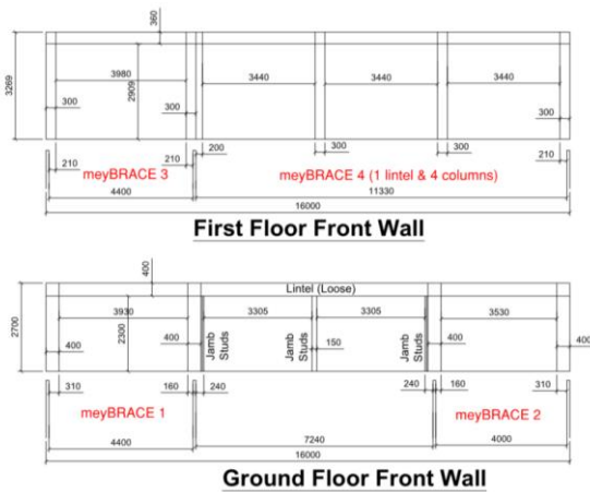
Front wall layout and meyBRACE locations
