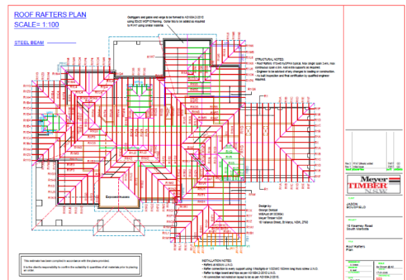
Roof Rafter Plan
