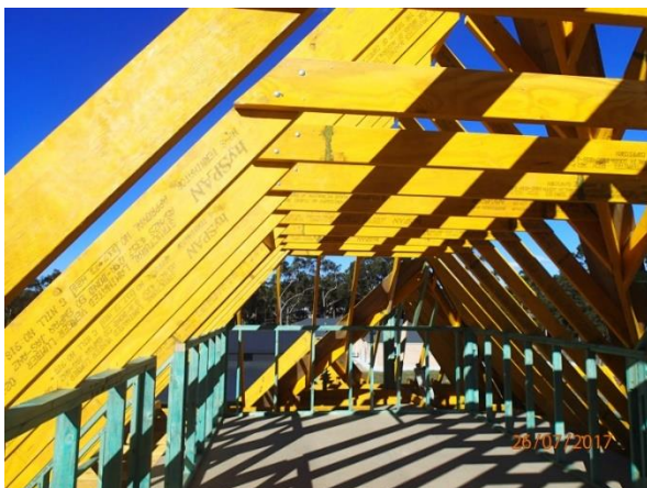
Loft with Rafters and Collar Ties
