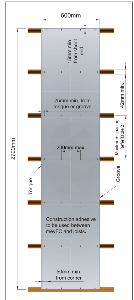
Figure 3: Fastener Layout
