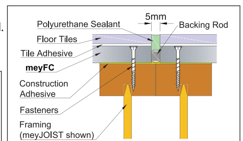
Figure 2: Control Joint
